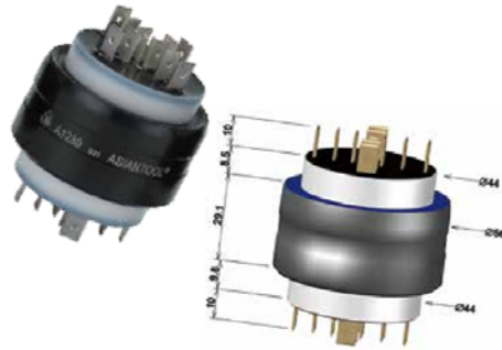
A1230 10poles/30A & 2poles/4A AC250V
